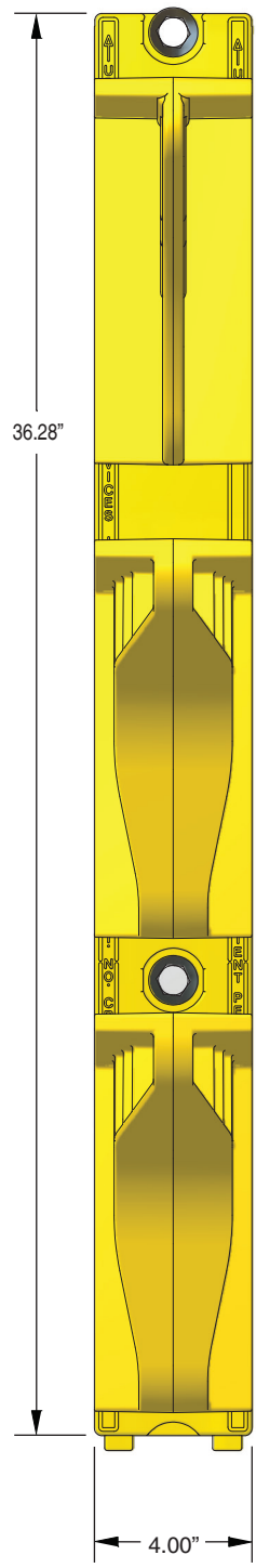
FRONT VIEW
